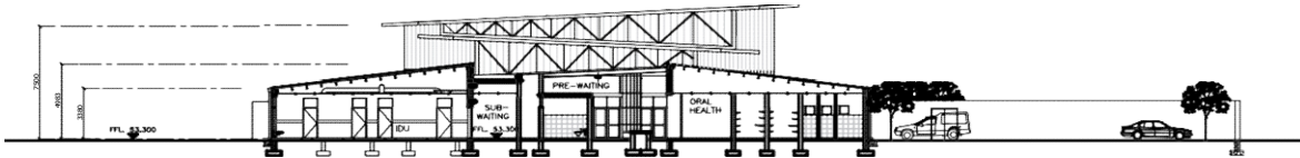
SECTION C - C
